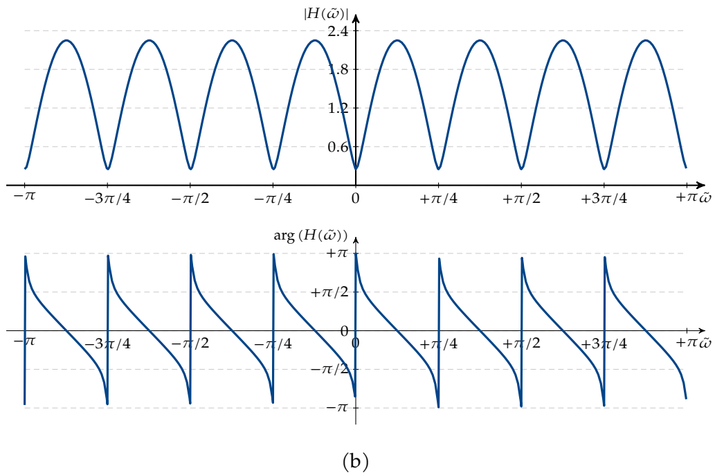
Figure 6.3: Frequency spectra of the feedforward comb filters of Figure 6.2 on the previous page, for the case q = 8 , with (a) a = 0.75 and (b) a = -1.25
