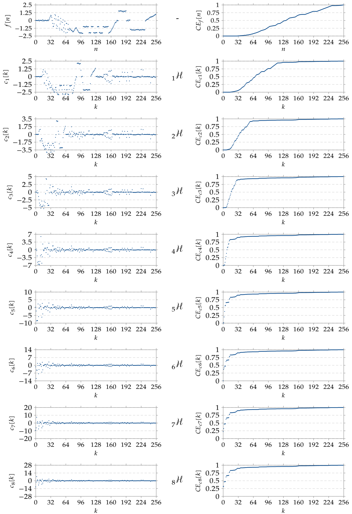
Figure 9.5: Example signal f[n] with its Haar transforms ( 1\mathcal{H} to 8\mathcal{H} ); the left column contains the (transformed) signal, the right column contains its cumulative energy distribution.
