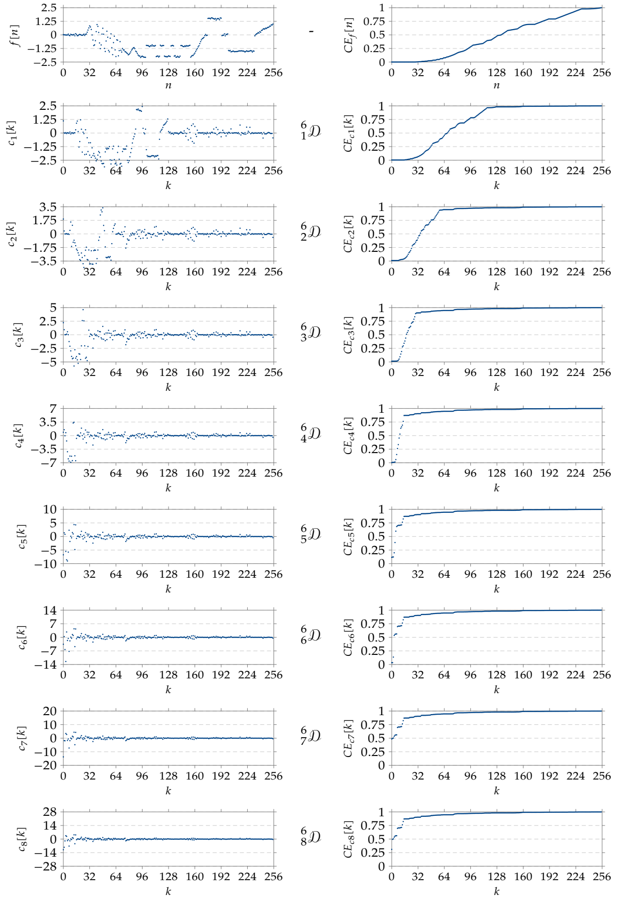
Figure 9.12: Example signal f[n] with its Daub-6 transforms ( {}^6_1\mathcal{D} to {}^6_8\mathcal{D} ); the left column contains the (transformed) signal, the right column contains its cumulative energy distribution.
