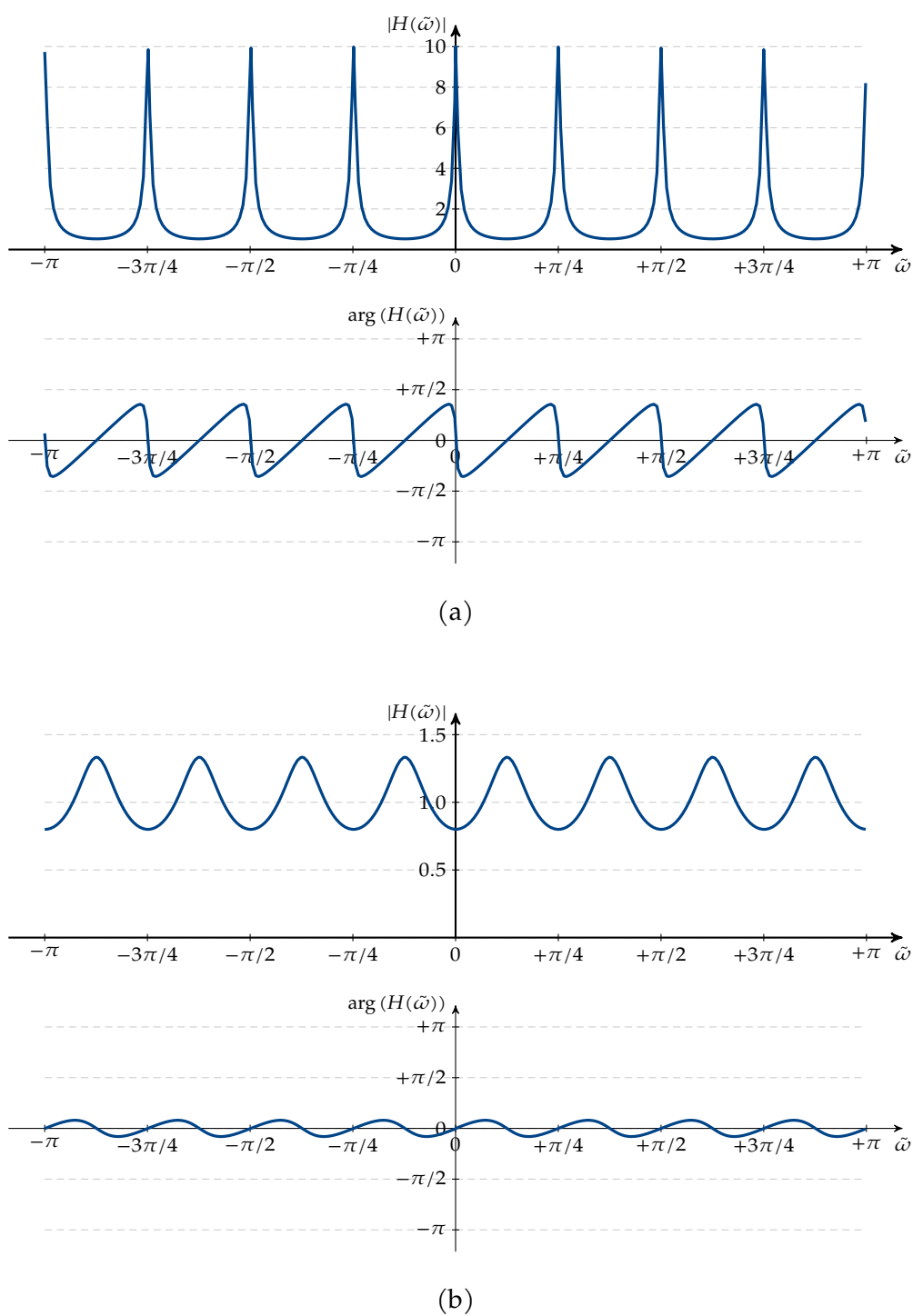
Figure 7.4: Frequency spectra of the feedback comb filters of Figure 7.3 on the facing page, for the case q = 8 , with (a) a = 0.9 and (b) a = -0.25
