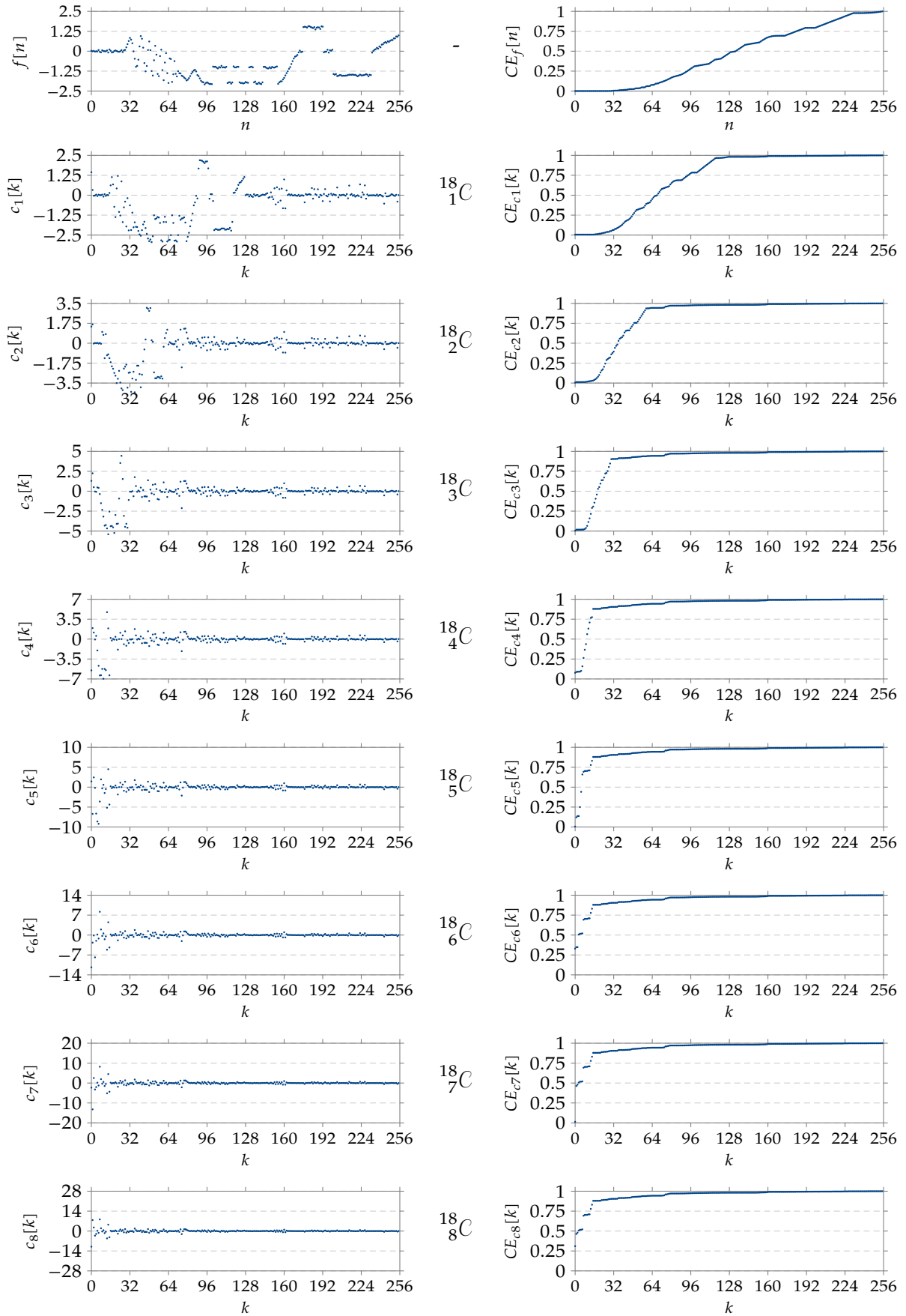
Figure 9.19: Example signal f[n] with its Coif-18 transforms ( {}^{18}_1C to {}^{18}_8C ); the left column contains the (transformed) signal, the right column contains its cumulative energy distribution.
