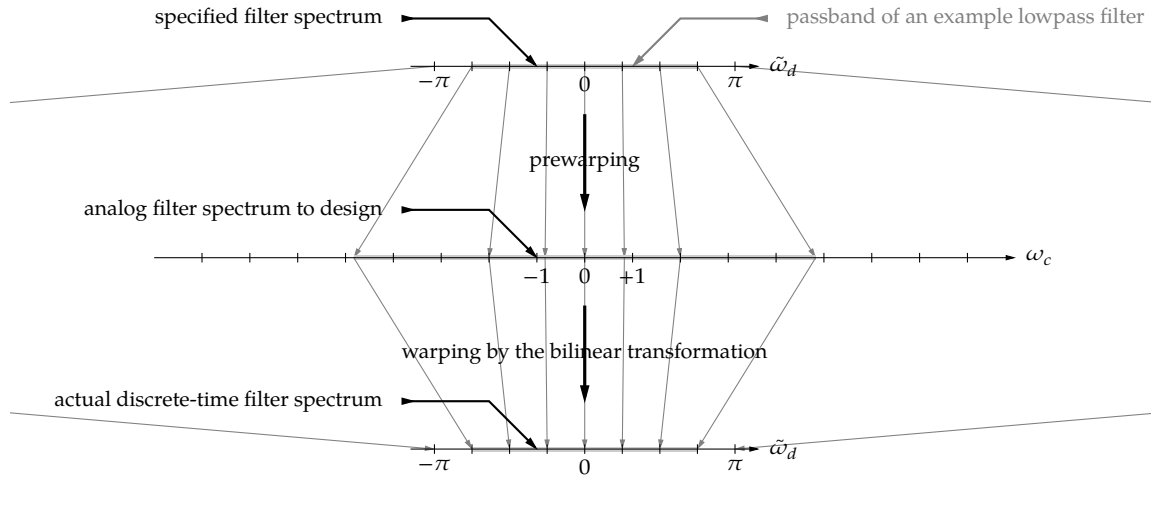
Figure 7.5: Illustration of the prewarping and warping effect related to the bilinear transformation
