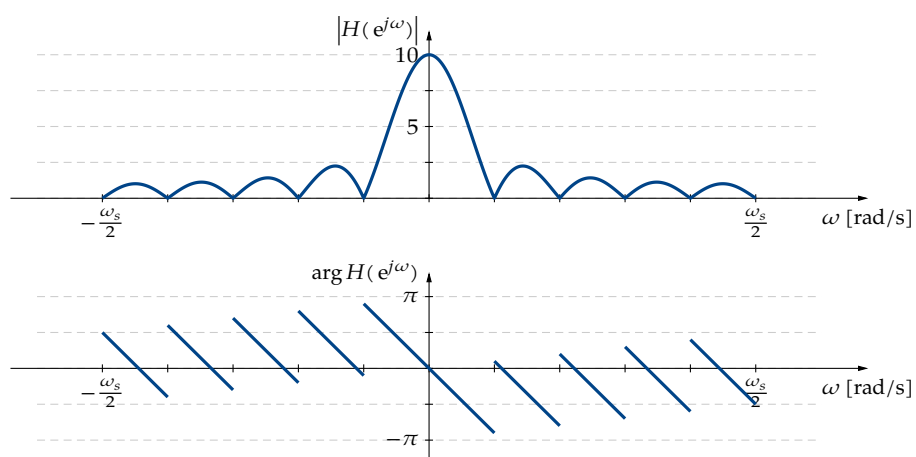
(b) Frequency response of the comb filter
